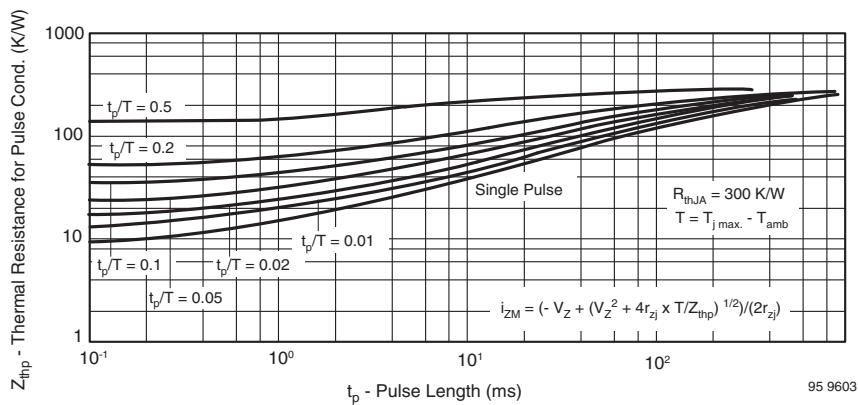
Fig. 10 - Thermal Response
