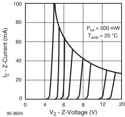
Fig. 7 - Z-Current vs. Z-Voltage
