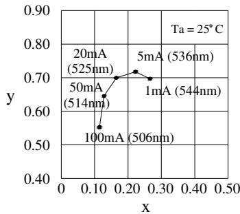
Forward Current vs. Chromaticity Coordinate ( \lambda D )
